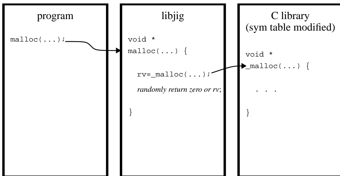
Figure 2: Intercepting calls to the memory allocation routine
